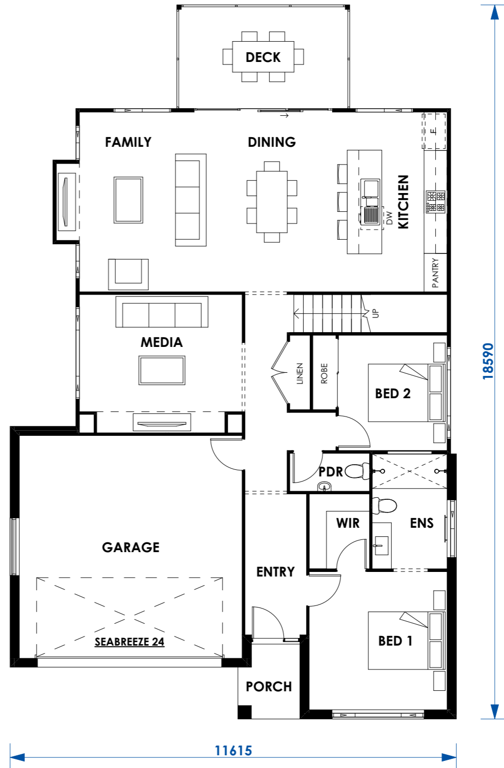
LEVEL 1 PLAN 1:100
